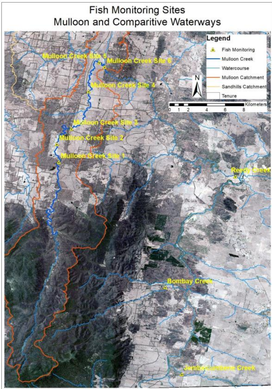
Figure 7. Map showing the reference sites in relation to the six Mulloon Creek sites.
