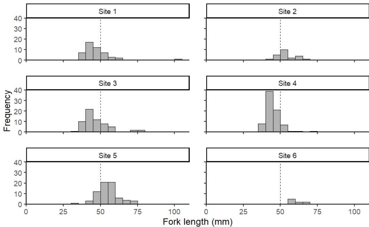
Figure 4. Length frequency of Mountain galaxias caught by backpack electrofishing in Mulloon Creek in May 2022. Dashed line indicates size at young-of-year (following O'Connor and Koehn 1991).
