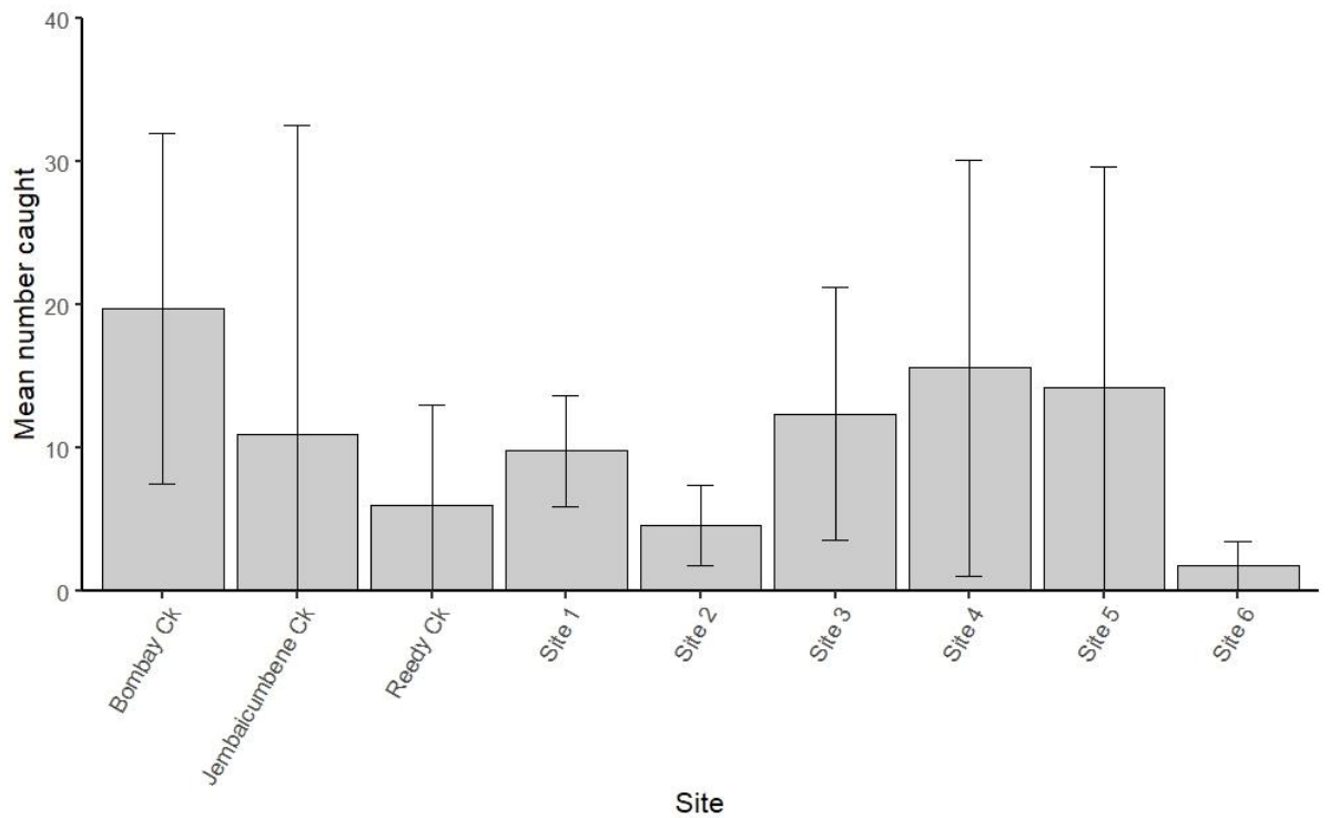
Figure 3. Mean number of Mountain galaxias caught per shot per site by backpack electrofishing May-June 2022. (Bars displayed as mean \pm 95% Confidence limits with Bonferroni correction).
