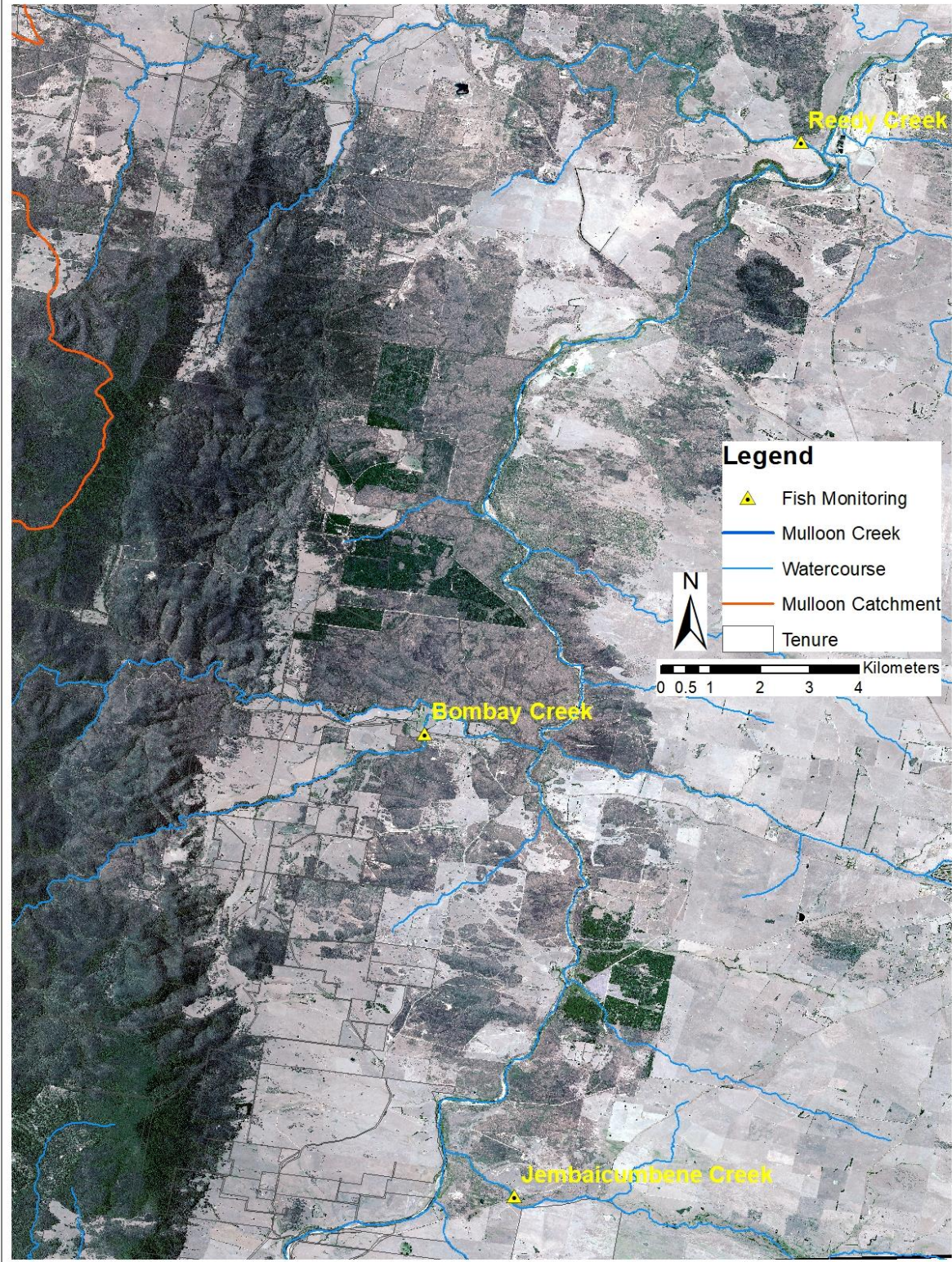
Figure 2. Map showing the three reference sampling locations outside the Mulloon catchment.
