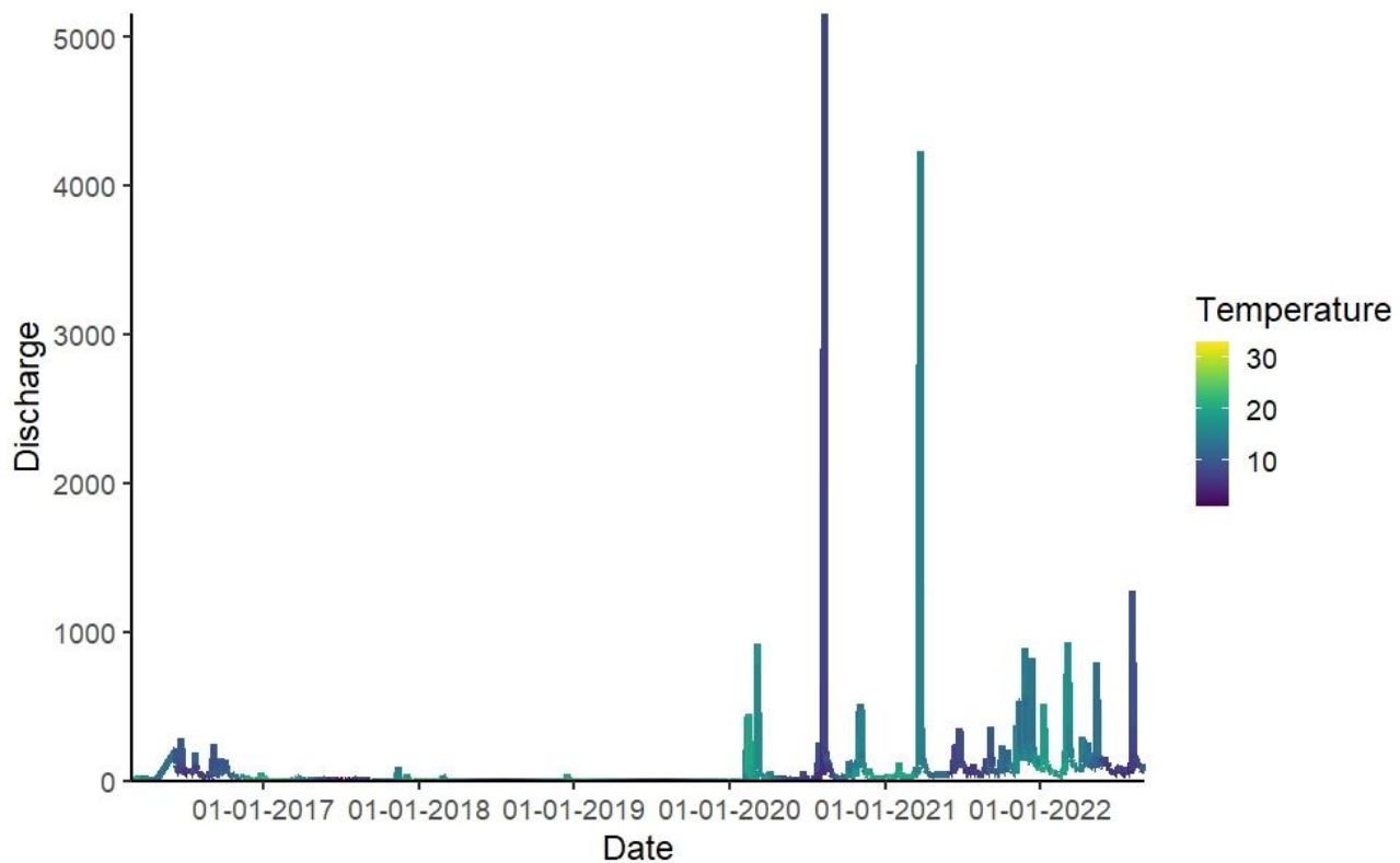
Figure 6. Daily discharge (ML/Day) and temperature of the Upper Mulloon Creek from March 2016 — September 2022.
