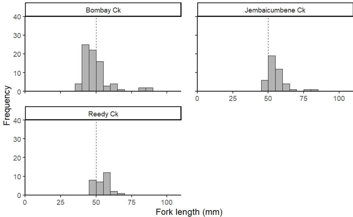
Figure 5. Length frequency of Mountain galaxias caught by backpack electrofishing from the three reference sites in June 2022. Dashed line indicates size at young-of-year (following O'Connor and Koehn 1991).
