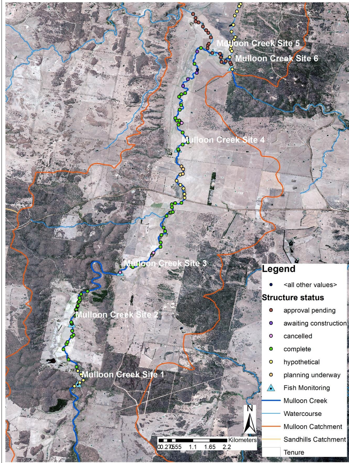
Figure 1. Map showing the six sampling locations and leaky weirs (green dots) along Mulloon Creek.
